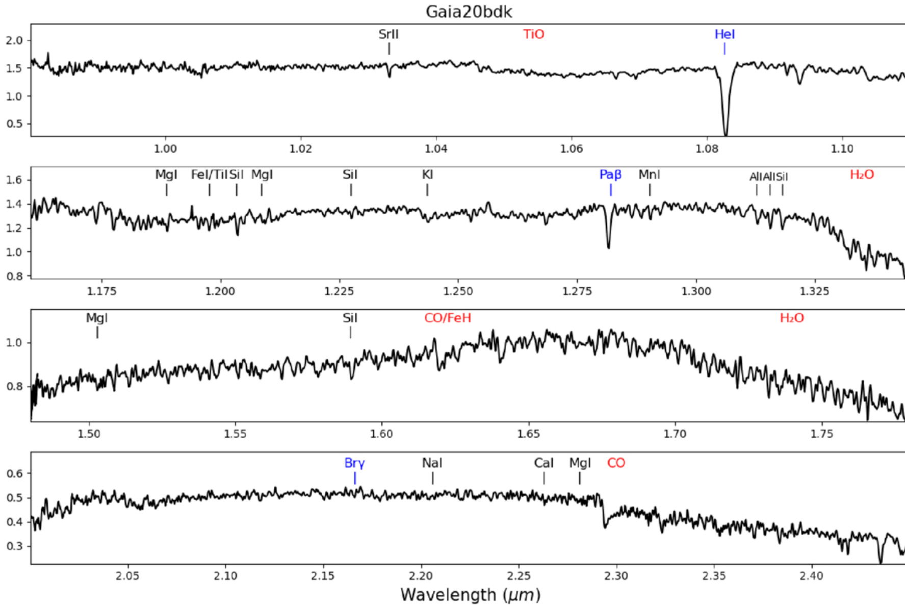
Figure 12. Dereddened spectra with all measured features labeled. from Evan R. Portnoi et al 2026 Astrophys. J. 1005 doi:10.3847/1538-4357/ae6dbc https://dx.doi.org/10.3847/1538-4357/ae6dbc © 2026. The Author(s). Published by the American Astronomical Society.
