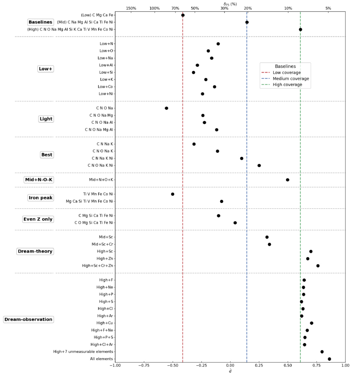
Figure 7. from Zhongyuan Zhang et al 2026 Astrophys. J. 1004 doi:10.3847/1538-4357/ae6dba https://dx.doi.org/10.3847/1538-4357/ae6dba © 2026. The Author(s). Published by the American Astronomical Society.
