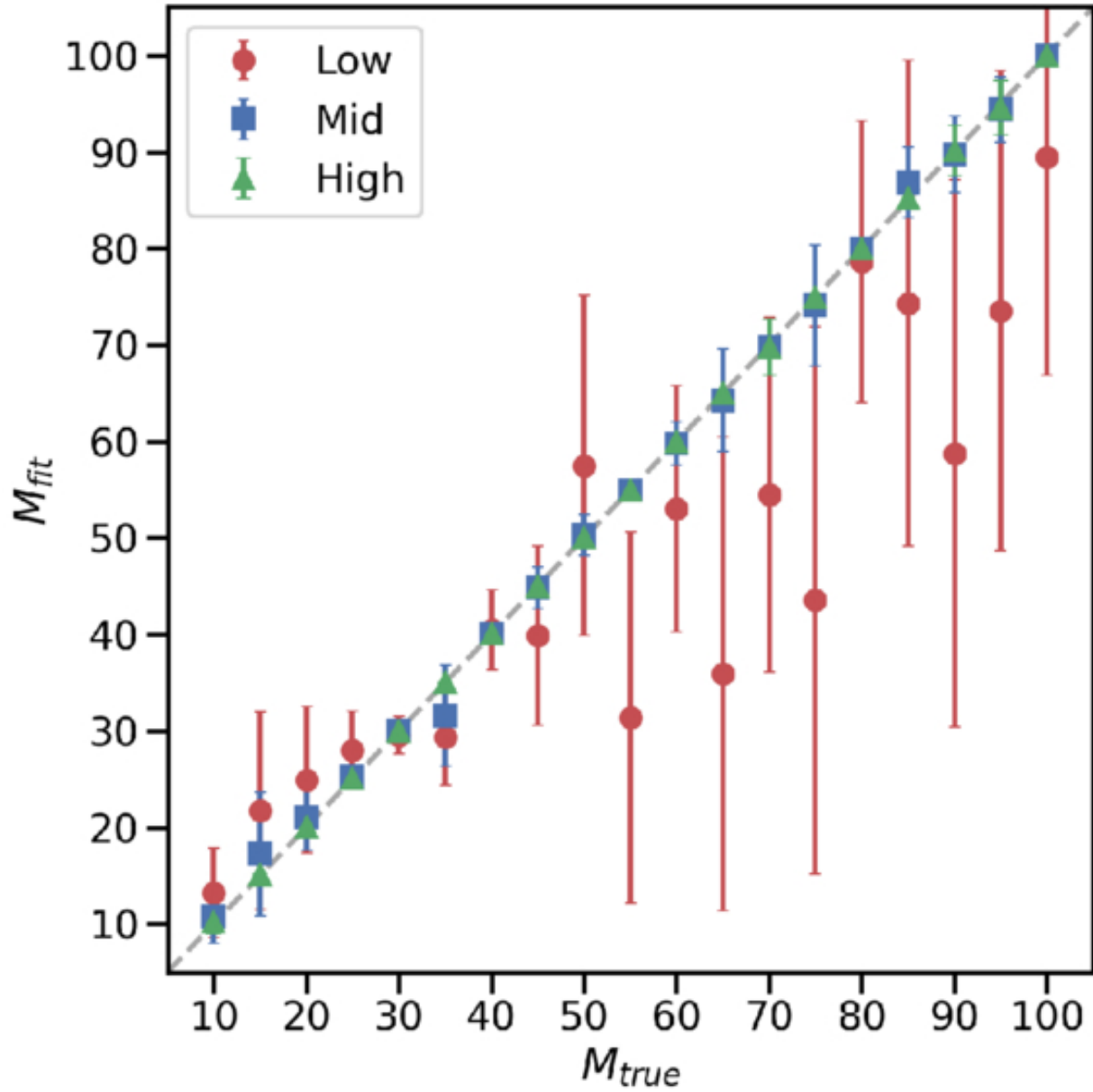
Figure 2. from Zhongyuan Zhang et al 2026 Astrophys. J. 1004 doi:10.3847/1538-4357/ae6dba https://dx.doi.org/10.3847/1538-4357/ae6dba © 2026. The Author(s). Published by the American Astronomical Society.
