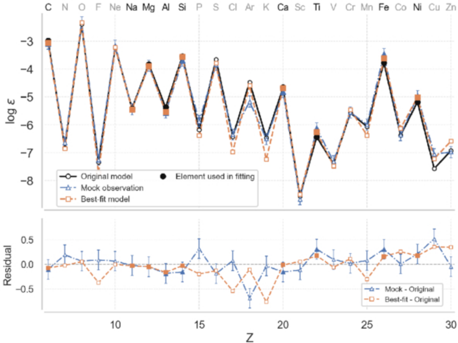
Figure 1. from Zhongyuan Zhang et al 2026 Astrophys. J. 1004 doi:10.3847/1538-4357/ae6dba https://dx.doi.org/10.3847/1538-4357/ae6dba © 2026. The Author(s). Published by the American Astronomical Society.
