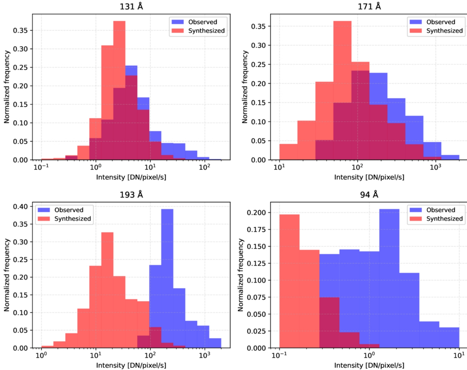
Figure 5. from Feng Chen 2026 Astrophys. J. 1004 doi:10.3847/1538-4357/ae6daa https://dx.doi.org/10.3847/1538-4357/ae6daa © 2026. The Author(s). Published by the American Astronomical Society.
