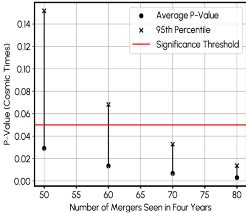
Figure 5. from Zachary J. Hoelscher et al 2026 Astrophys. J. 1004 doi:10.3847/1538-4357/ae6ced https://dx.doi.org/10.3847/1538-4357/ae6ced © 2026. The Author(s). Published by the American Astronomical Society.
