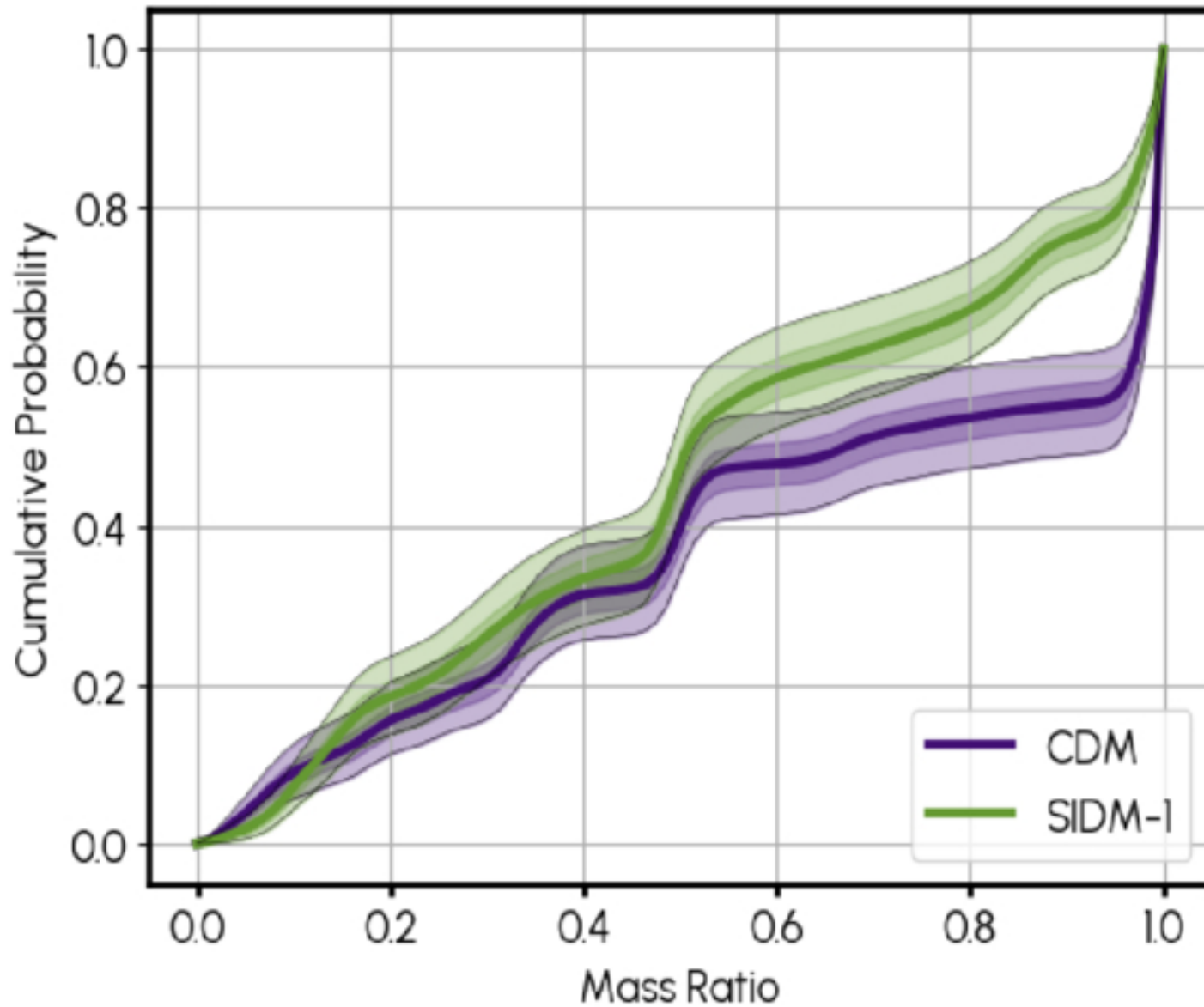
Figure 4. from Zachary J. Hoelscher et al 2026 Astrophys. J. 1004 doi:10.3847/1538-4357/ae6ced https://dx.doi.org/10.3847/1538-4357/ae6ced © 2026. The Author(s). Published by the American Astronomical Society.
