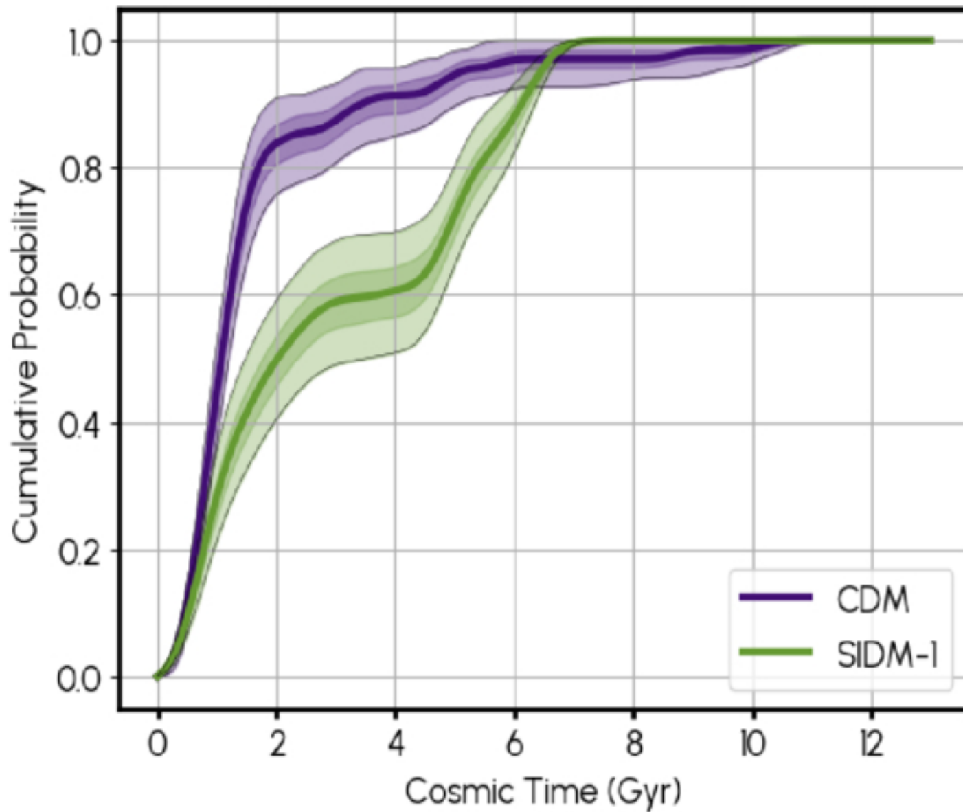
Figure 3. from Zachary J. Hoelscher et al 2026 Astrophys. J. 1004 doi:10.3847/1538-4357/ae6ced https://dx.doi.org/10.3847/1538-4357/ae6ced © 2026. The Author(s). Published by the American Astronomical Society.
