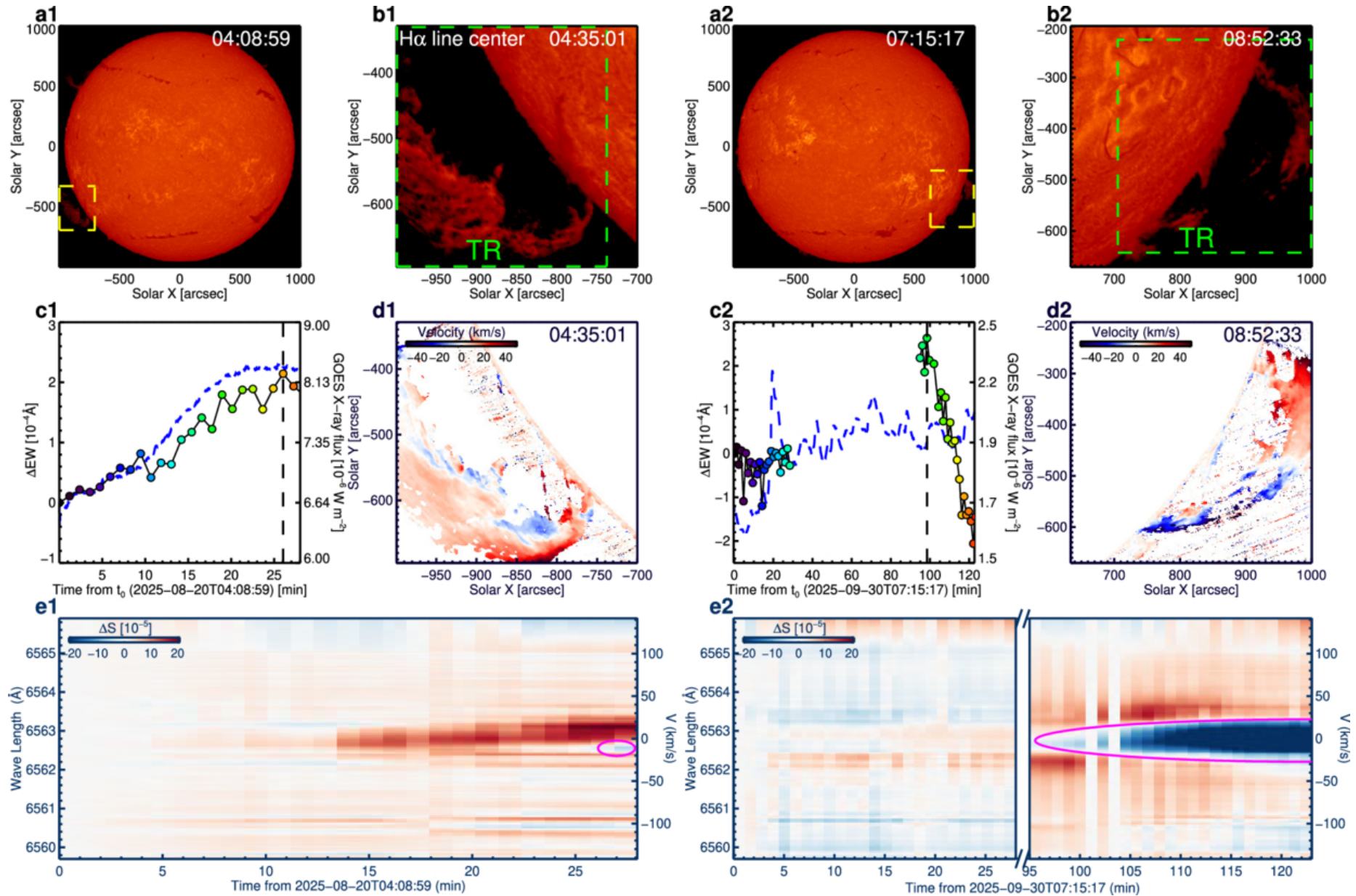
Figure 4. from Junyi Zhang et al 2026 Astrophys. J. 1004 doi:10.3847/1538-4357/ae6c22 https://dx.doi.org/10.3847/1538-4357/ae6c22 © 2026. The Author(s). Published by the American Astronomical Society.
