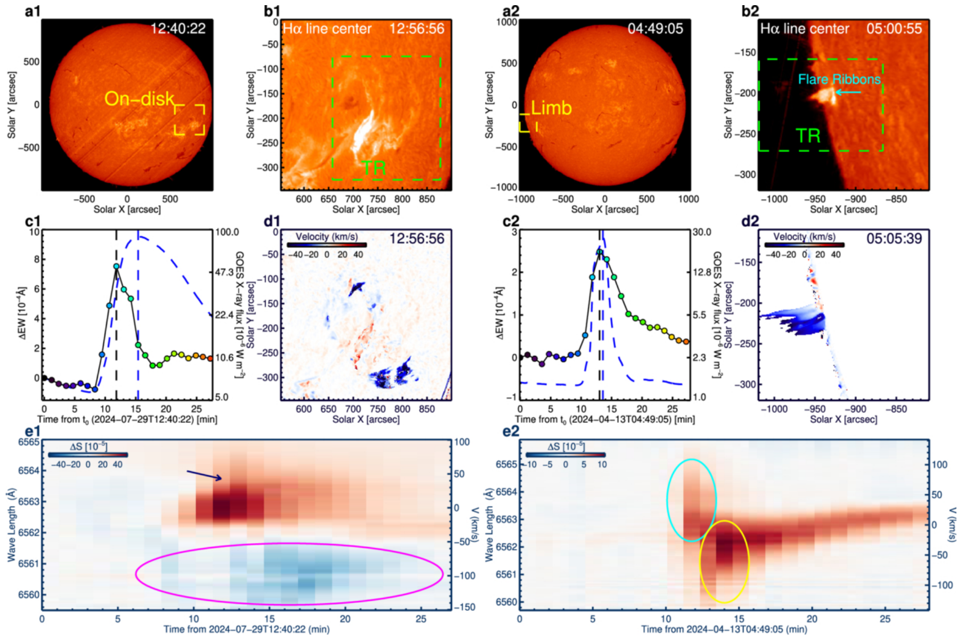
Figure 1. from Junyi Zhang et al 2026 Astrophys. J. 1004 doi:10.3847/1538-4357/ae6c22 https://dx.doi.org/10.3847/1538-4357/ae6c22 © 2026. The Author(s). Published by the American Astronomical Society.
