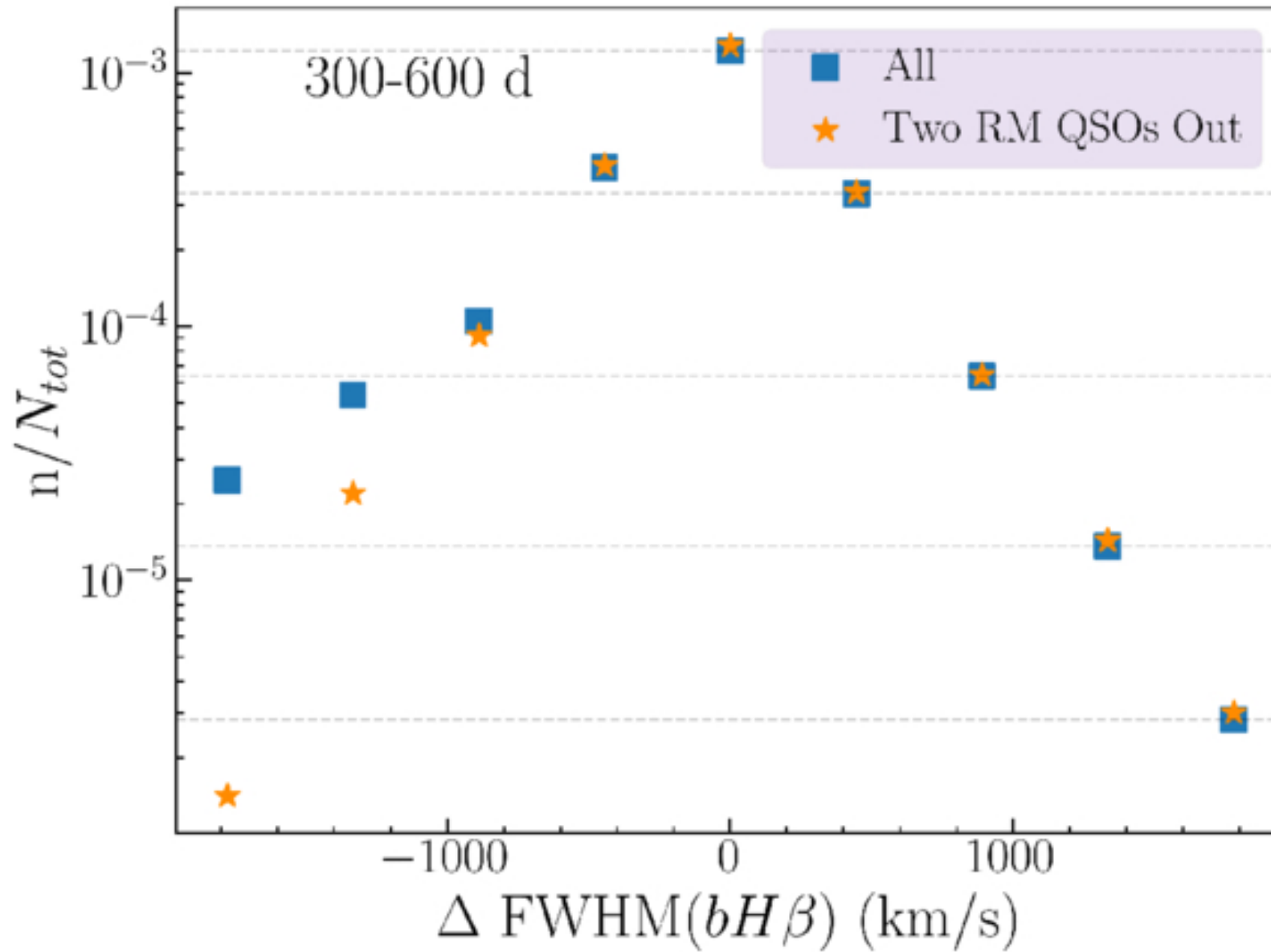
Figure 9. from Collin M. Dabbieri et al 2026 Astrophys. J. 1005 doi:10.3847/1538-4357/ae6c1f https://dx.doi.org/10.3847/1538-4357/ae6c1f © 2026. The Author(s). Published by the American Astronomical Society.
