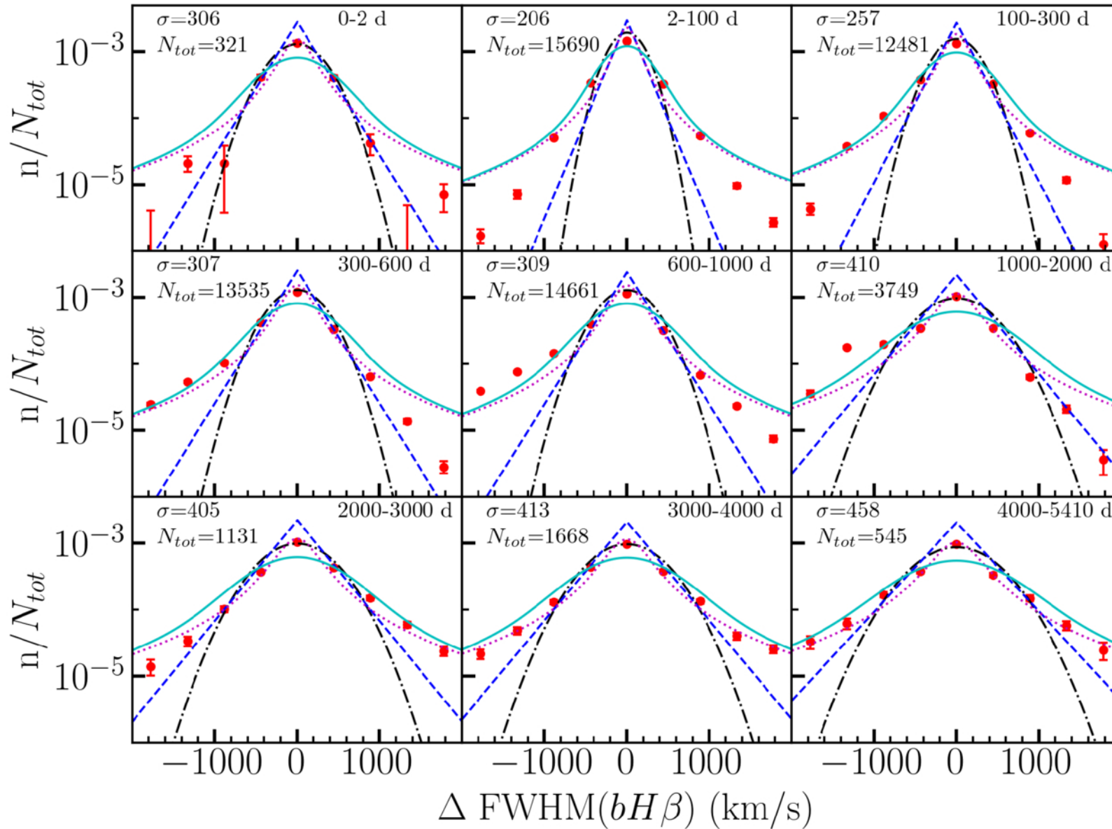
Figure 8. from Collin M. Dabbieri et al 2026 Astrophys. J. 1005 doi:10.3847/1538-4357/ae6c1f https://dx.doi.org/10.3847/1538-4357/ae6c1f © 2026. The Author(s). Published by the American Astronomical Society.
