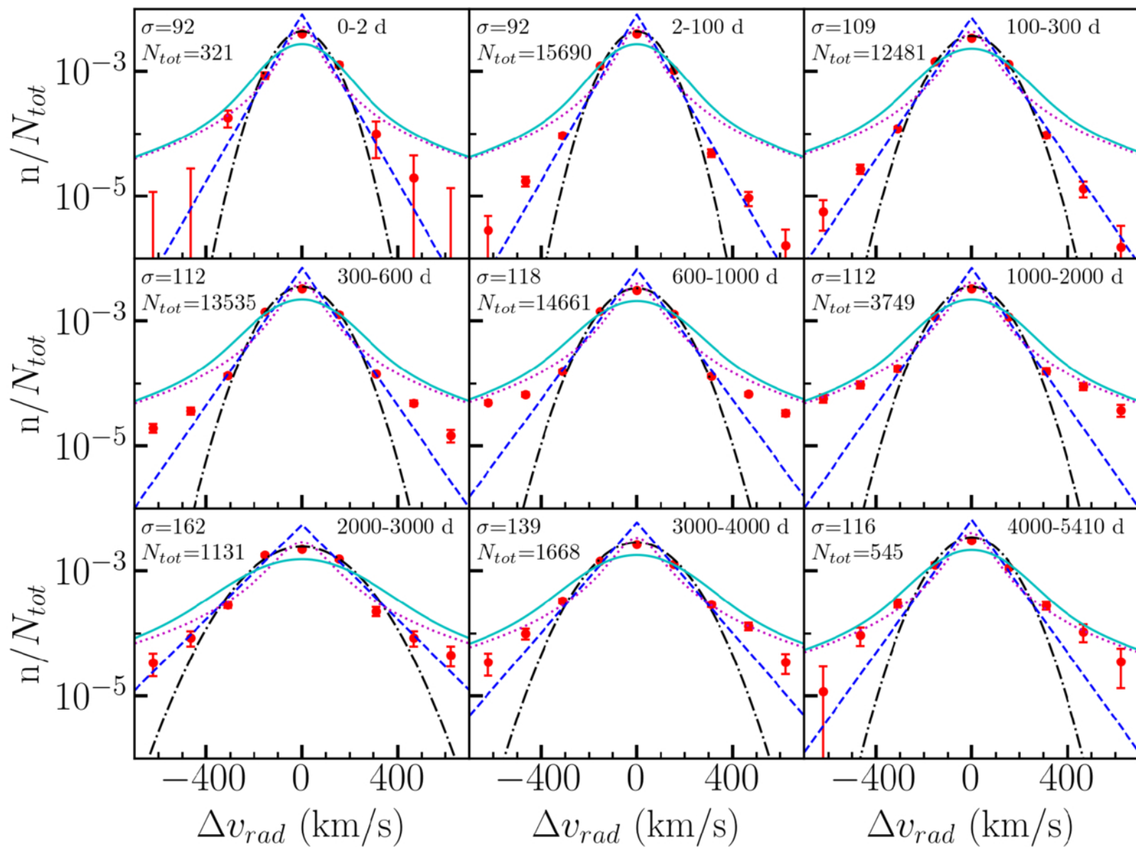
Figure 7. Variability Histograms from Collin M. Dabbieri et al 2026 Astrophys. J. 1005 doi:10.3847/1538-4357/ae6c1f https://dx.doi.org/10.3847/1538-4357/ae6c1f © 2026. The Author(s). Published by the American Astronomical Society.
