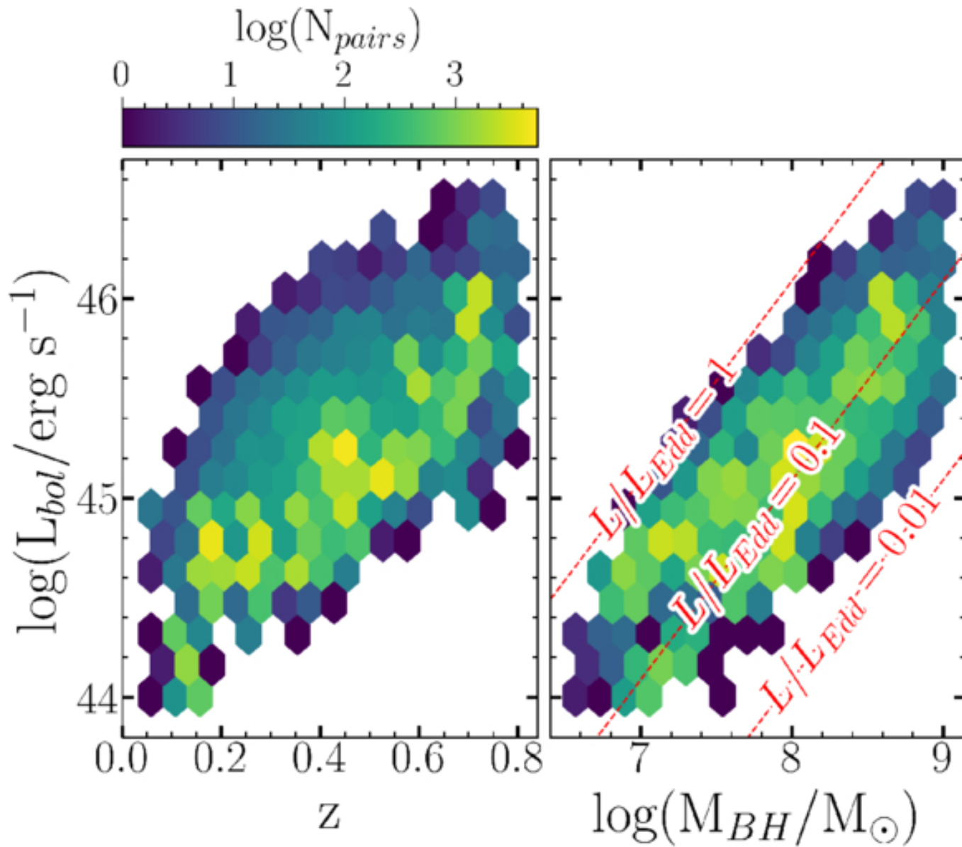
Figure 4. from Collin M. Dabbieri et al 2026 Astrophys. J. 1005 doi:10.3847/1538-4357/ae6c1f https://dx.doi.org/10.3847/1538-4357/ae6c1f © 2026. The Author(s). Published by the American Astronomical Society.
