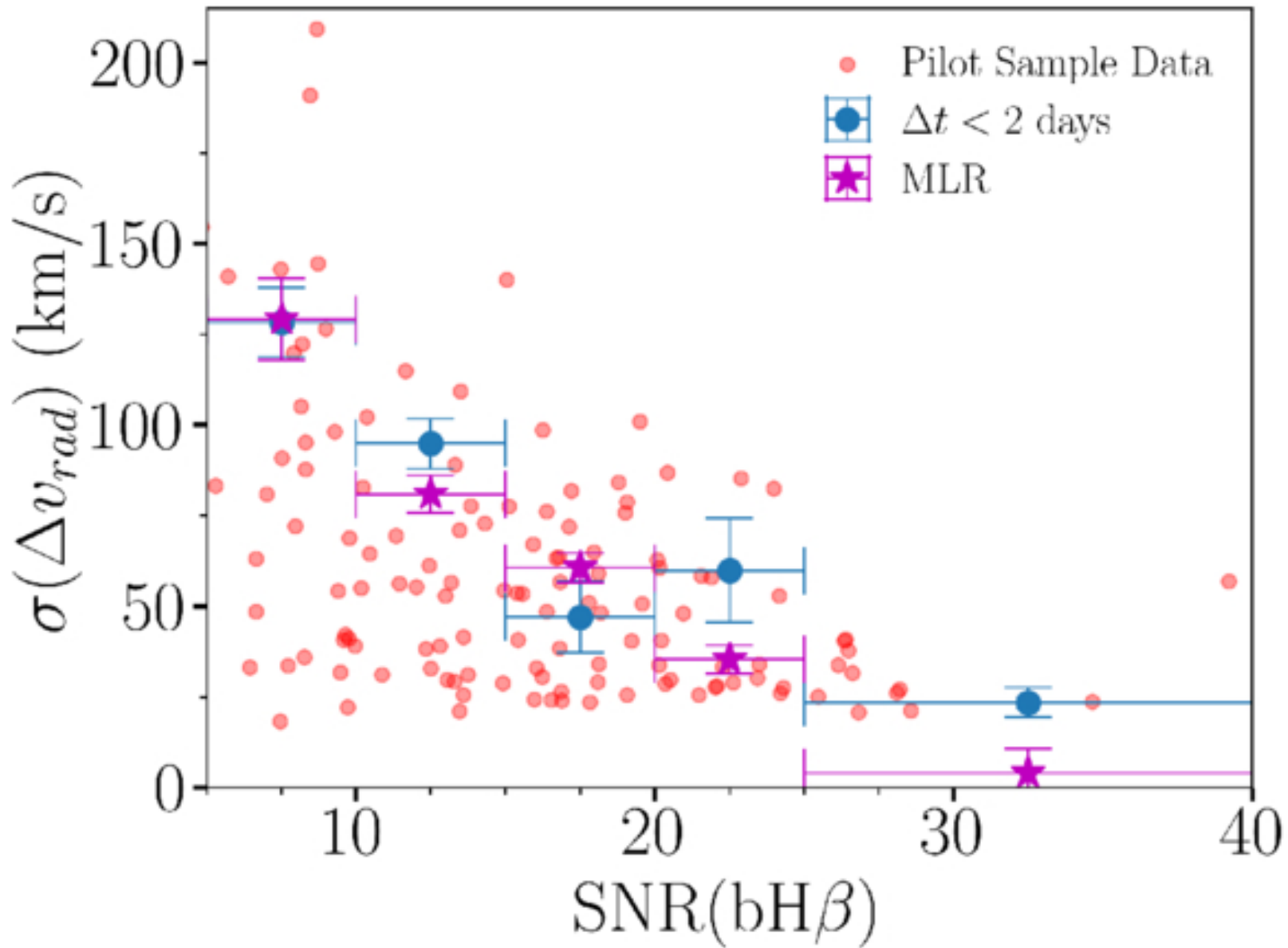
Figure 3. from Collin M. Dabbieri et al 2026 Astrophys. J. 1005 doi:10.3847/1538-4357/ae6c1f https://dx.doi.org/10.3847/1538-4357/ae6c1f © 2026. The Author(s). Published by the American Astronomical Society.
