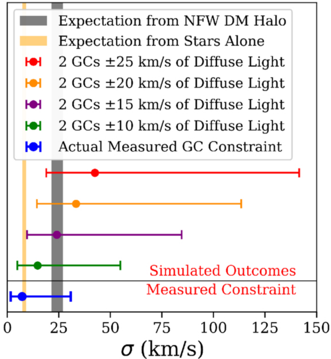
Figure 5. from Michael A. Keim et al 2026 Astrophys. J. 1004 doi:10.3847/1538-4357/ae6b8d https://dx.doi.org/10.3847/1538-4357/ae6b8d © 2026. The Author(s). Published by the American Astronomical Society.
