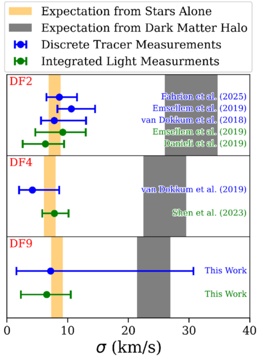
Figure 3. from Michael A. Keim et al 2026 Astrophys. J. 1004 doi:10.3847/1538-4357/ae6b8d https://dx.doi.org/10.3847/1538-4357/ae6b8d © 2026. The Author(s). Published by the American Astronomical Society.
