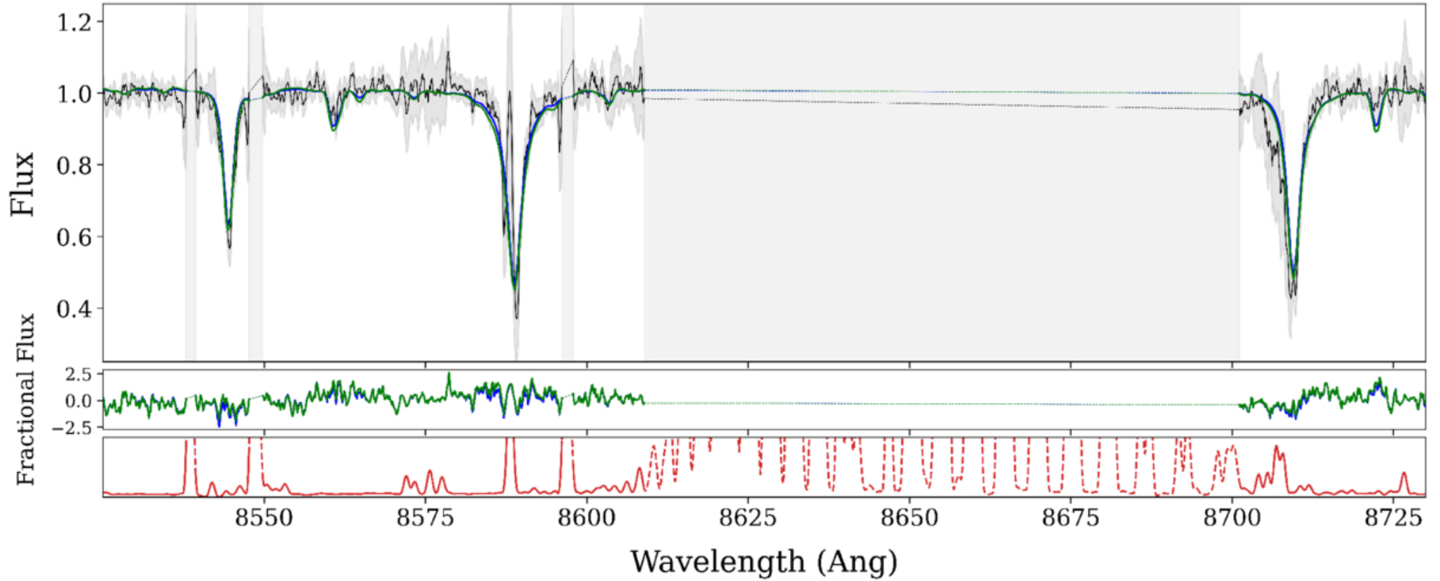
Figure 2. from Michael A. Keim et al 2026 Astrophys. J. 1004 doi:10.3847/1538-4357/ae6b8d https://dx.doi.org/10.3847/1538-4357/ae6b8d © 2026. The Author(s). Published by the American Astronomical Society.
