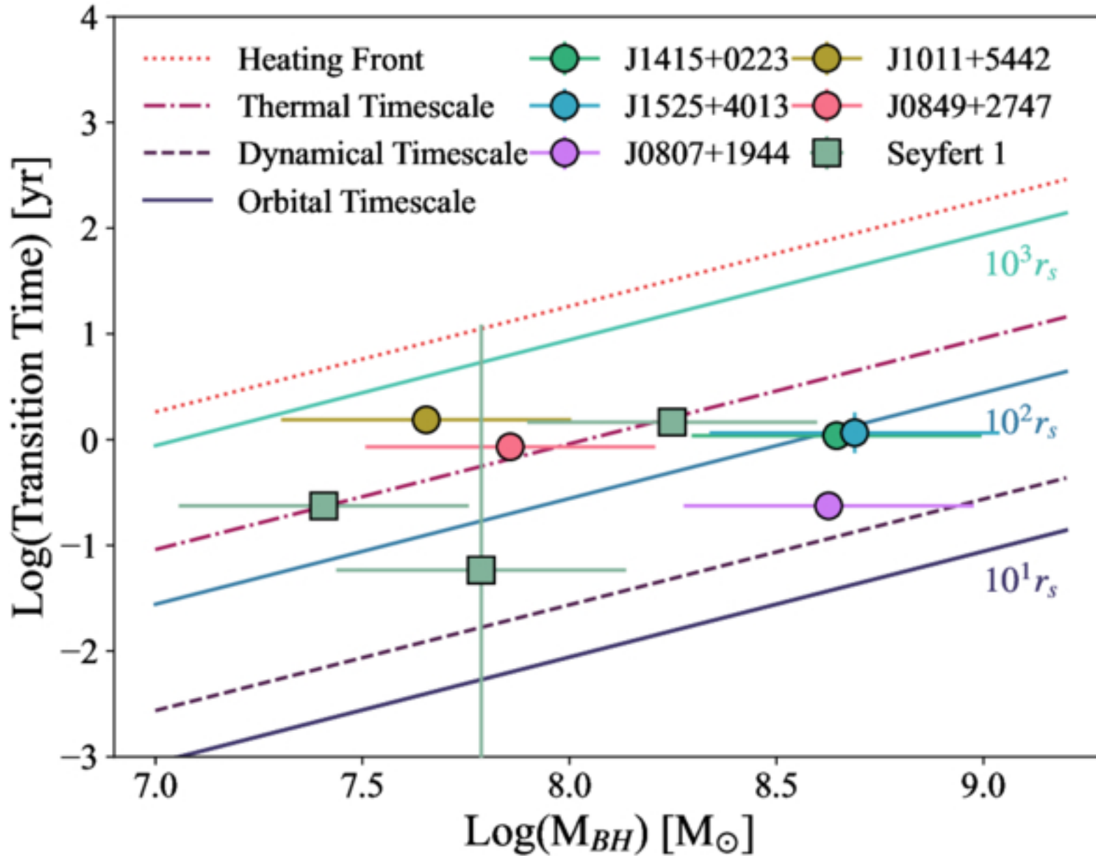
Figure 9. from Margaret E. Verrico et al 2026 Astrophys. J. 1004 doi:10.3847/1538-4357/ae6b77 https://dx.doi.org/10.3847/1538-4357/ae6b77 © 2026. The Author(s). Published by the American Astronomical Society.
