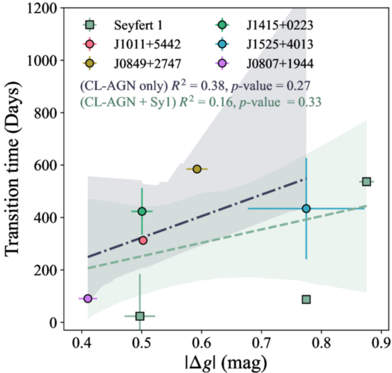
Figure 8. from Margaret E. Verrico et al 2026 Astrophys. J. 1004 doi:10.3847/1538-4357/ae6b77 https://dx.doi.org/10.3847/1538-4357/ae6b77 © 2026. The Author(s). Published by the American Astronomical Society.
