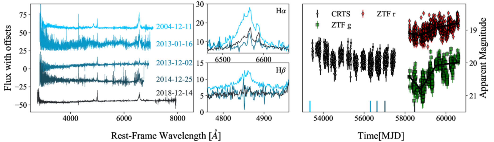
Figure 6. from Margaret E. Verrico et al 2026 Astrophys. J. 1004 doi:10.3847/1538-4357/ae6b77 https://dx.doi.org/10.3847/1538-4357/ae6b77 © 2026. The Author(s). Published by the American Astronomical Society.
