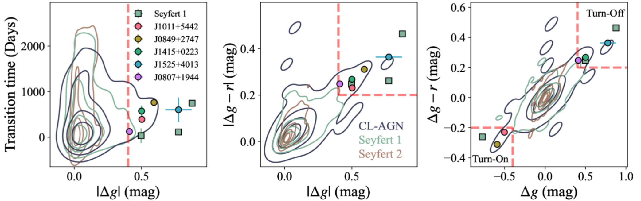
Figure 5. from Margaret E. Verrico et al 2026 Astrophys. J. 1004 doi:10.3847/1538-4357/ae6b77 https://dx.doi.org/10.3847/1538-4357/ae6b77 © 2026. The Author(s). Published by the American Astronomical Society.
