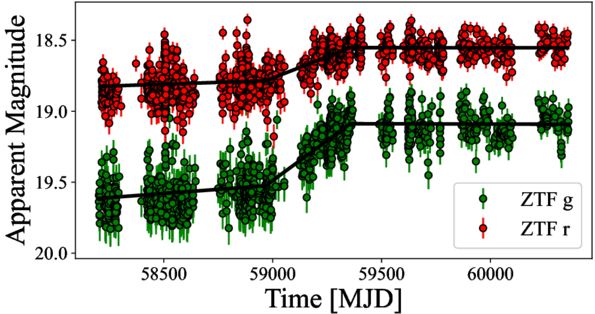
Figure 1. from Margaret E. Verrico et al 2026 Astrophys. J. 1004 doi:10.3847/1538-4357/ae6b77 https://dx.doi.org/10.3847/1538-4357/ae6b77 © 2026. The Author(s). Published by the American Astronomical Society.
