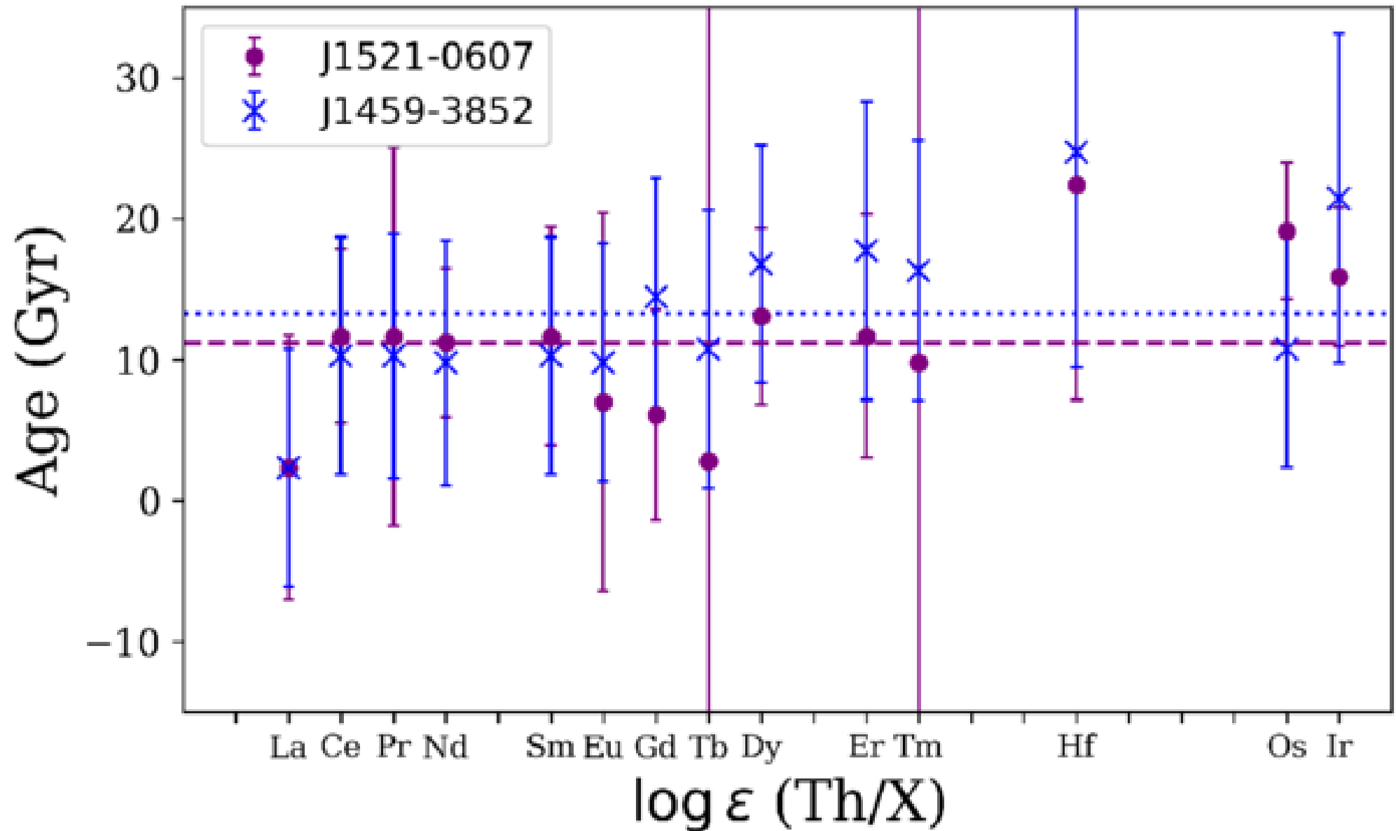
Figure 5. from Jessica Merritt Agnos et al 2026 Astrophys. J. 1004 doi:10.3847/1538-4357/ae6b72 https://dx.doi.org/10.3847/1538-4357/ae6b72 © 2026. The Author(s). Published by the American Astronomical Society.
