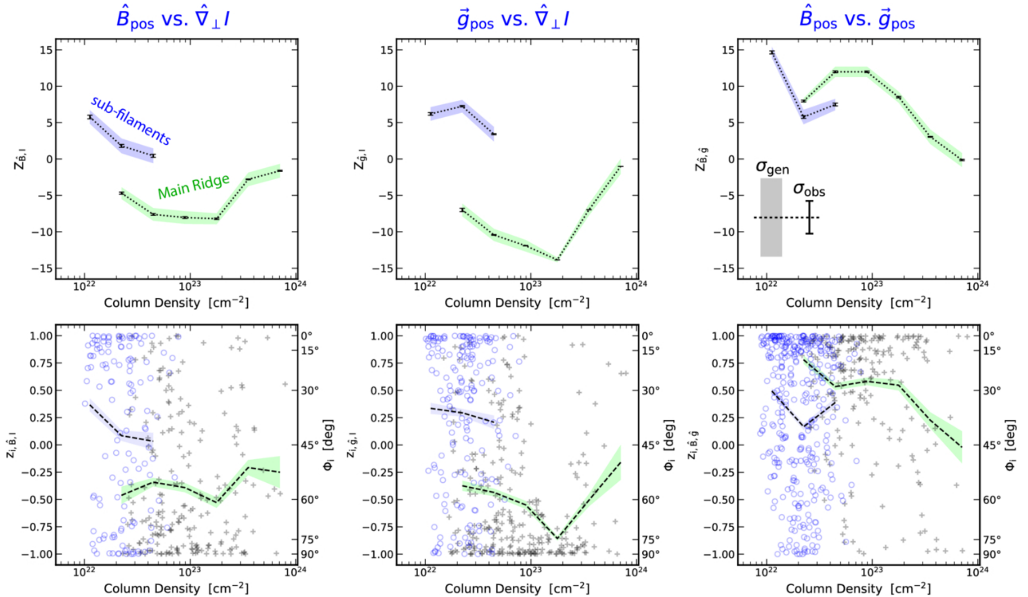
Figure 5. from Thushara G. S. Pillai et al 2026 Astrophys. J. 1004 doi:10.3847/1538-4357/ae6a97 https://dx.doi.org/10.3847/1538-4357/ae6a97 © 2026. The Author(s). Published by the American Astronomical Society.
