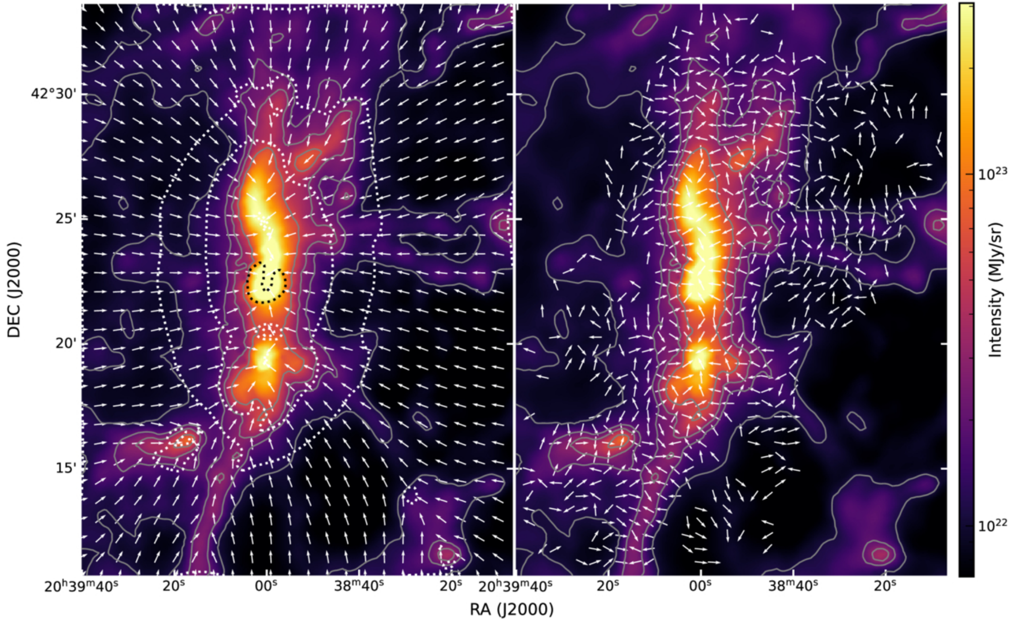
Figure 4. from Thushara G. S. Pillai et al 2026 Astrophys. J. 1004 doi:10.3847/1538-4357/ae6a97 https://dx.doi.org/10.3847/1538-4357/ae6a97 © 2026. The Author(s). Published by the American Astronomical Society.
