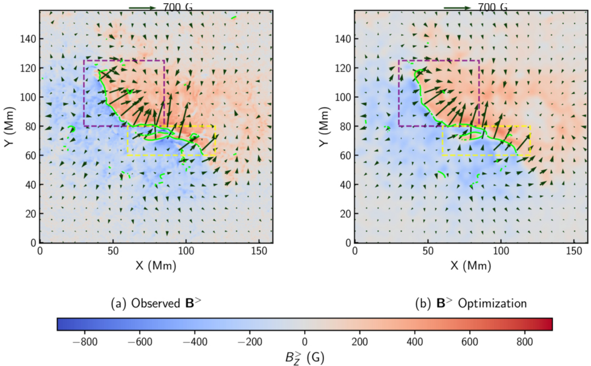
Figure 9. from Abhinav G. Iyer et al 2026 Astrophys. J. 1004 doi:10.3847/1538-4357/ae6a8b https://dx.doi.org/10.3847/1538-4357/ae6a8b © 2026. The Author(s). Published by the American Astronomical Society.
