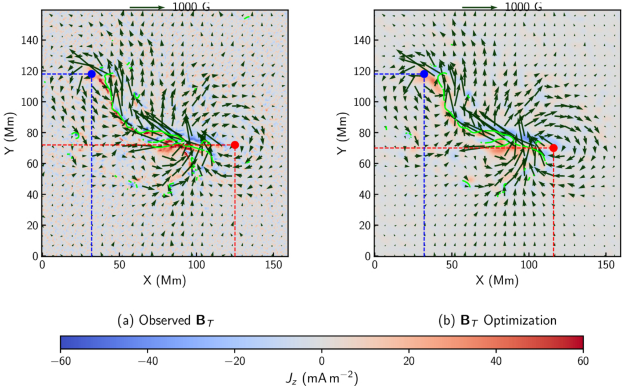
Figure 11. from Abhinav G. Iyer et al 2026 Astrophys. J. 1004 doi:10.3847/1538-4357/ae6a8b https://dx.doi.org/10.3847/1538-4357/ae6a8b © 2026. The Author(s). Published by the American Astronomical Society.
