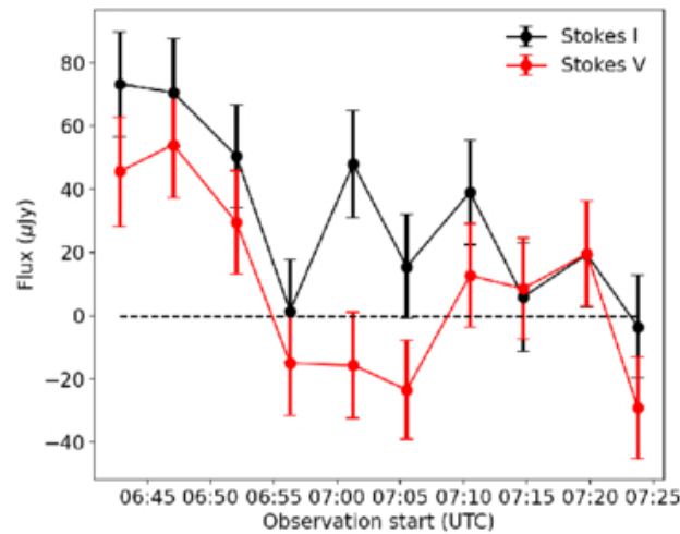
(d) The 8–12 GHz light curve of UZ For on October 19.
