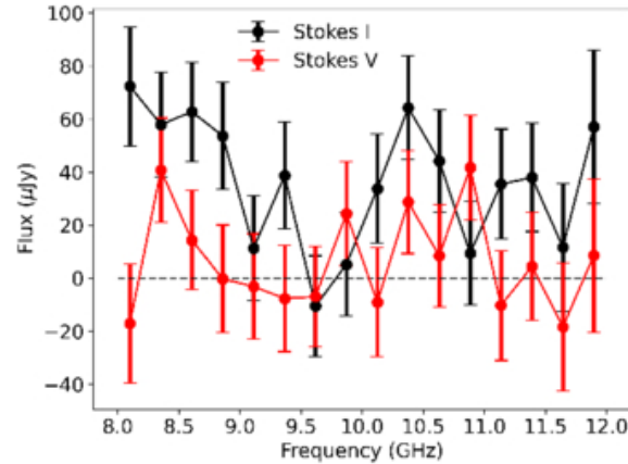
(b) The 8–12 GHz SED of UZ For on October 19.
