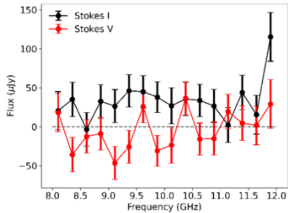
(a) The 8–12 GHz SED of UZ For on October 17.
