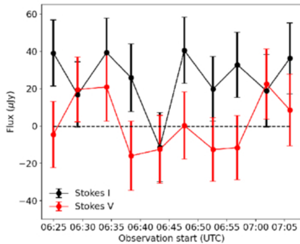
(c) The 8–12 GHz light curve of UZ For on October 17.
