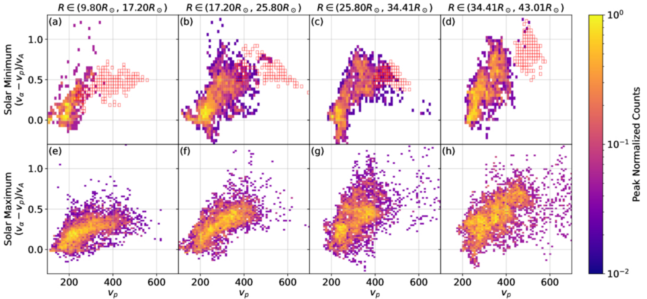
Figure 4. from Shuyi Meng and Shuo Yao 2026 Astrophys. J. 1004 doi:10.3847/1538-4357/ae69c9 https://dx.doi.org/10.3847/1538-4357/ae69c9 © 2026. The Author(s). Published by the American Astronomical Society.
