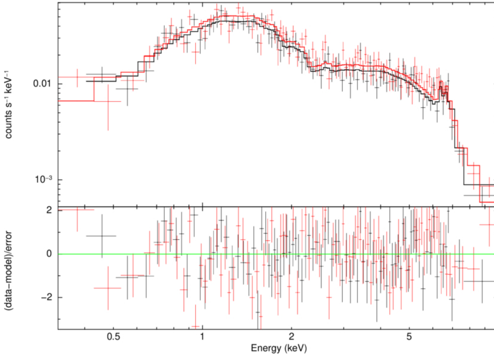
Figure 8. from Fang-Zhou Yan et al 2026 Astrophys. J. 1003 doi:10.3847/1538-4357/ae6913 https://dx.doi.org/10.3847/1538-4357/ae6913 © 2026. The Author(s). Published by the American Astronomical Society.
