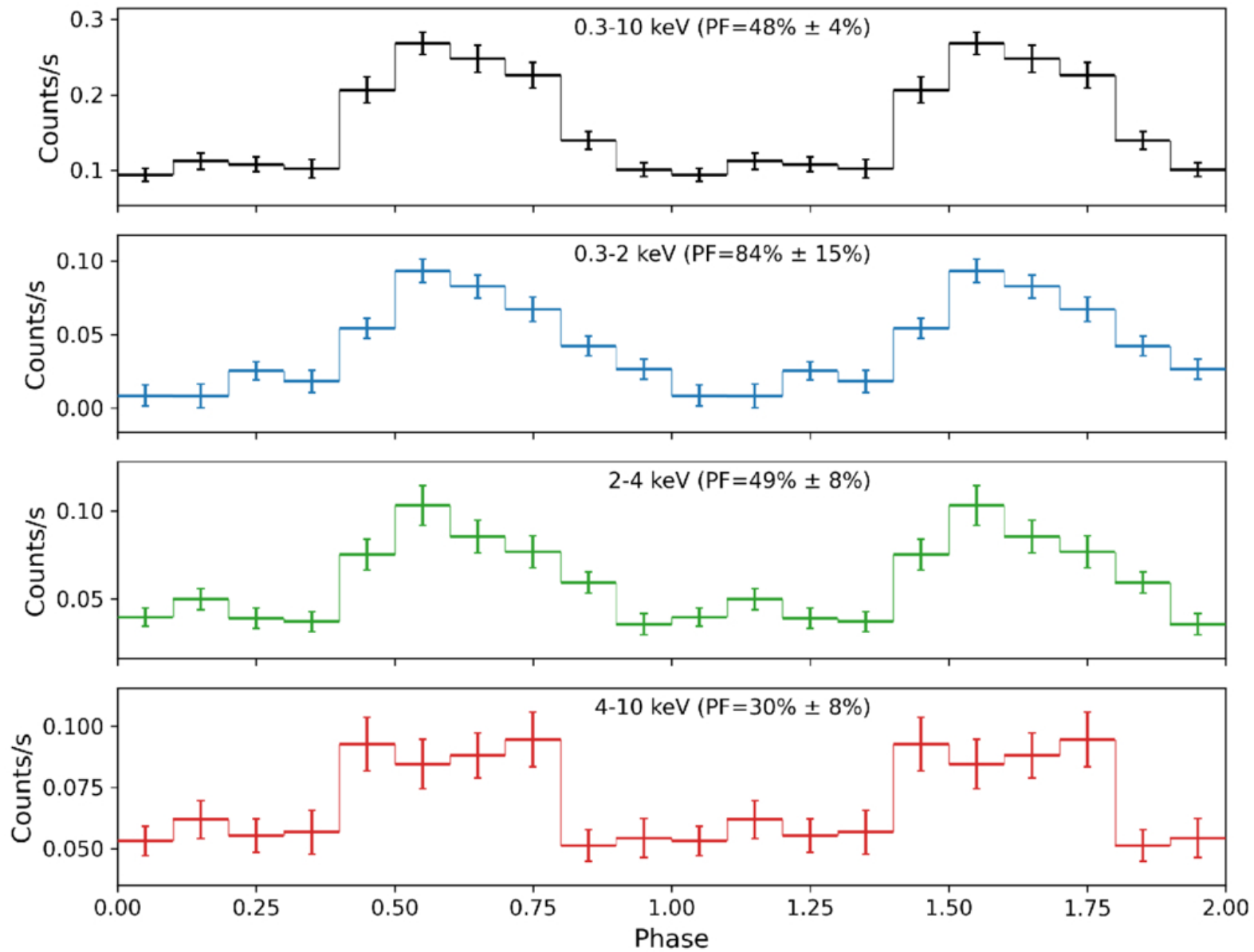
Figure 7. from Fang-Zhou Yan et al 2026 Astrophys. J. 1003 doi:10.3847/1538-4357/ae6913 https://dx.doi.org/10.3847/1538-4357/ae6913 © 2026. The Author(s). Published by the American Astronomical Society.
