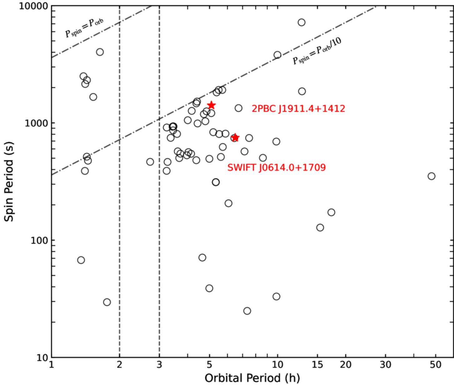
Figure 10. from Fang-Zhou Yan et al 2026 Astrophys. J. 1003 doi:10.3847/1538-4357/ae6913 https://dx.doi.org/10.3847/1538-4357/ae6913 © 2026. The Author(s). Published by the American Astronomical Society.
