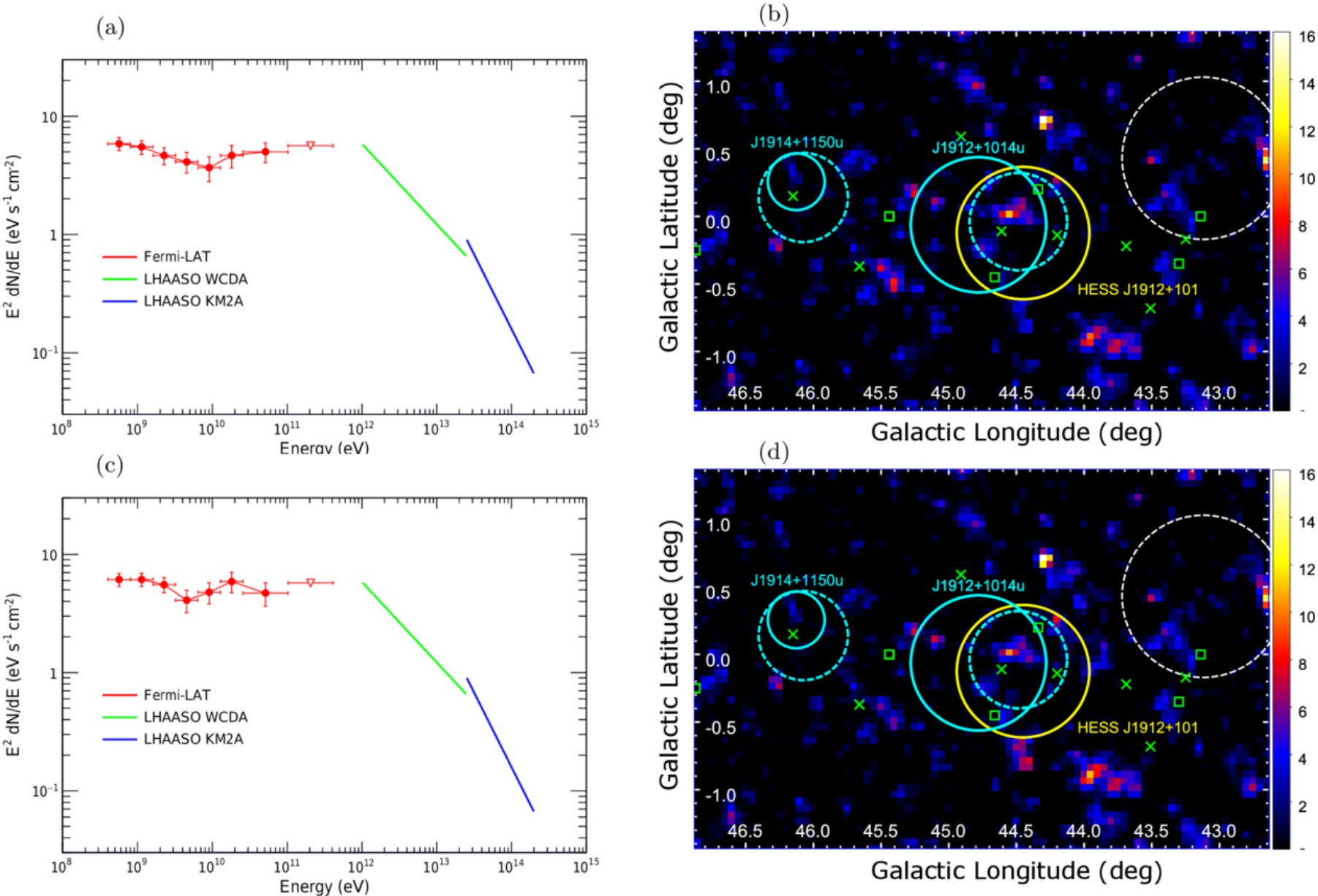
Figure 9. from Tsunefumi Mizuno et al 2026 Astrophys. J. 1006 doi:10.3847/1538-4357/ae680d https://dx.doi.org/10.3847/1538-4357/ae680d © 2026. The Author(s). Published by the American Astronomical Society.
