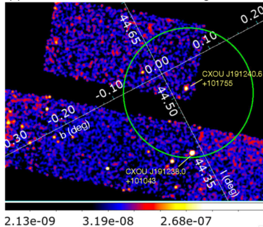
(a) Chandra ACIS 0.5–5.0 keV image
