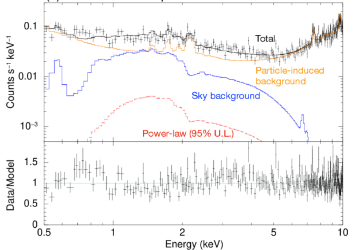
(b) Chandra ACIS spectrum
