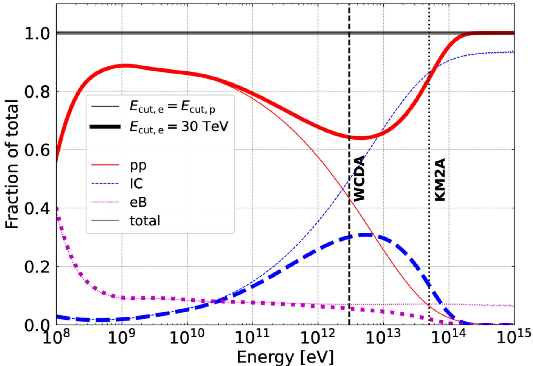
Figure 6. from Tsunefumi Mizuno et al 2026 Astrophys. J. 1006 doi:10.3847/1538-4357/ae680d https://dx.doi.org/10.3847/1538-4357/ae680d © 2026. The Author(s). Published by the American Astronomical Society.
