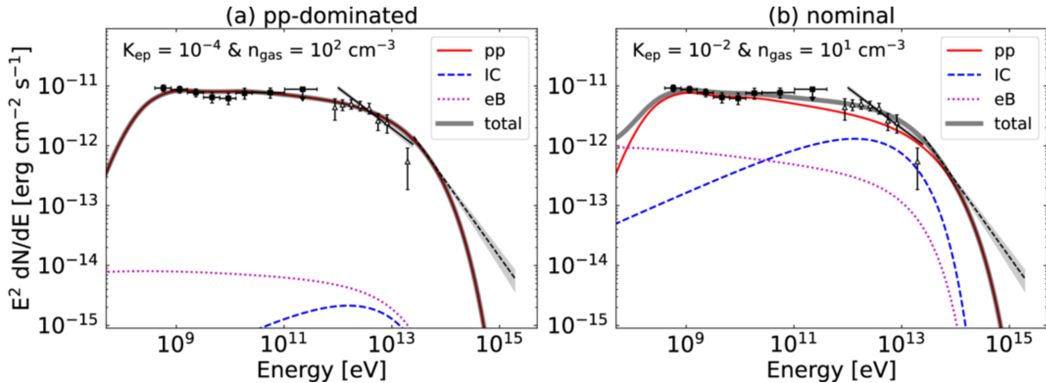
Figure 5. from Tsunefumi Mizuno et al 2026 Astrophys. J. 1006 doi:10.3847/1538-4357/ae680d https://dx.doi.org/10.3847/1538-4357/ae680d © 2026. The Author(s). Published by the American Astronomical Society.
