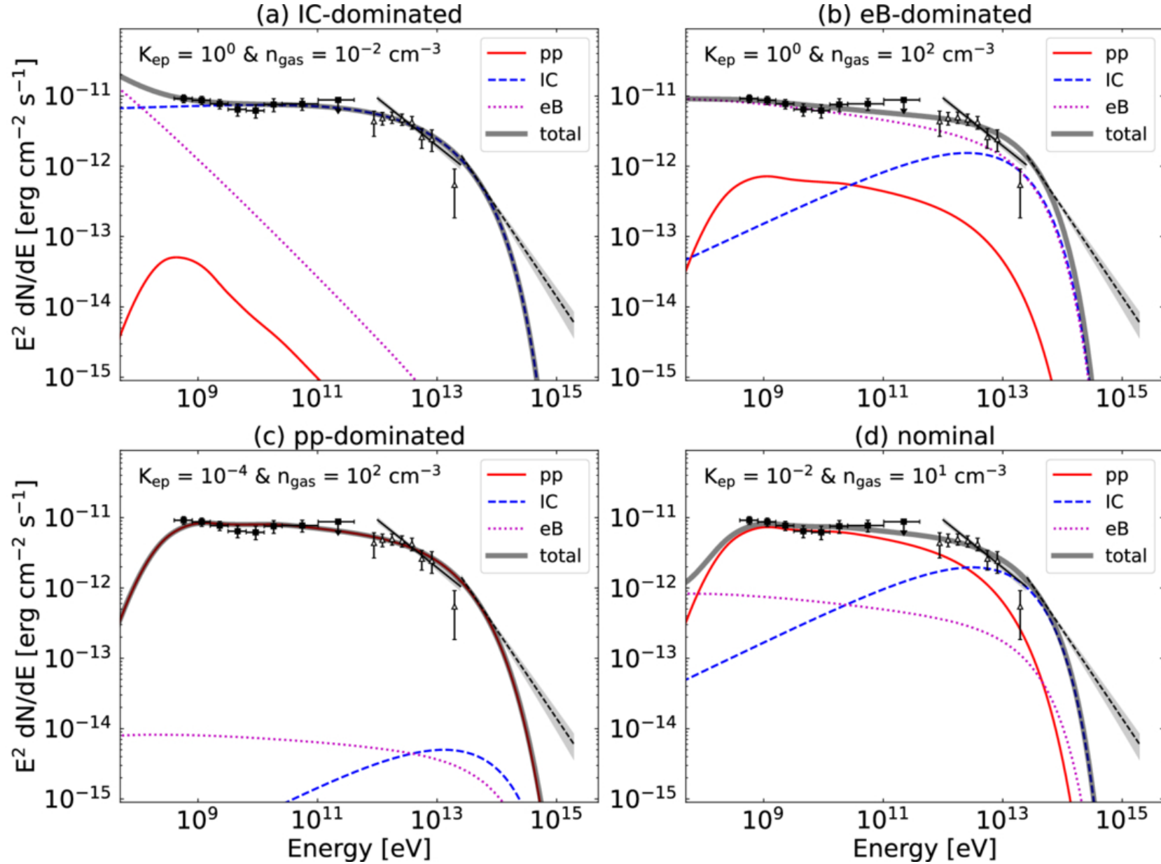
Figure 4. from Tsunefumi Mizuno et al 2026 Astrophys. J. 1006 doi:10.3847/1538-4357/ae680d https://dx.doi.org/10.3847/1538-4357/ae680d © 2026. The Author(s). Published by the American Astronomical Society.
