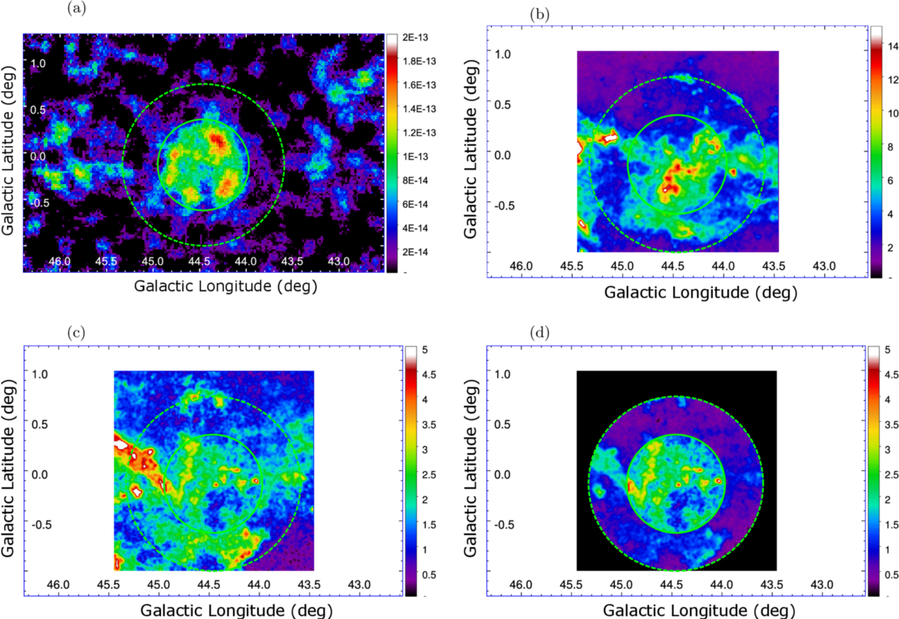
Figure 2. from Tsunefumi Mizuno et al 2026 Astrophys. J. 1006 doi:10.3847/1538-4357/ae680d https://dx.doi.org/10.3847/1538-4357/ae680d © 2026. The Author(s). Published by the American Astronomical Society.
