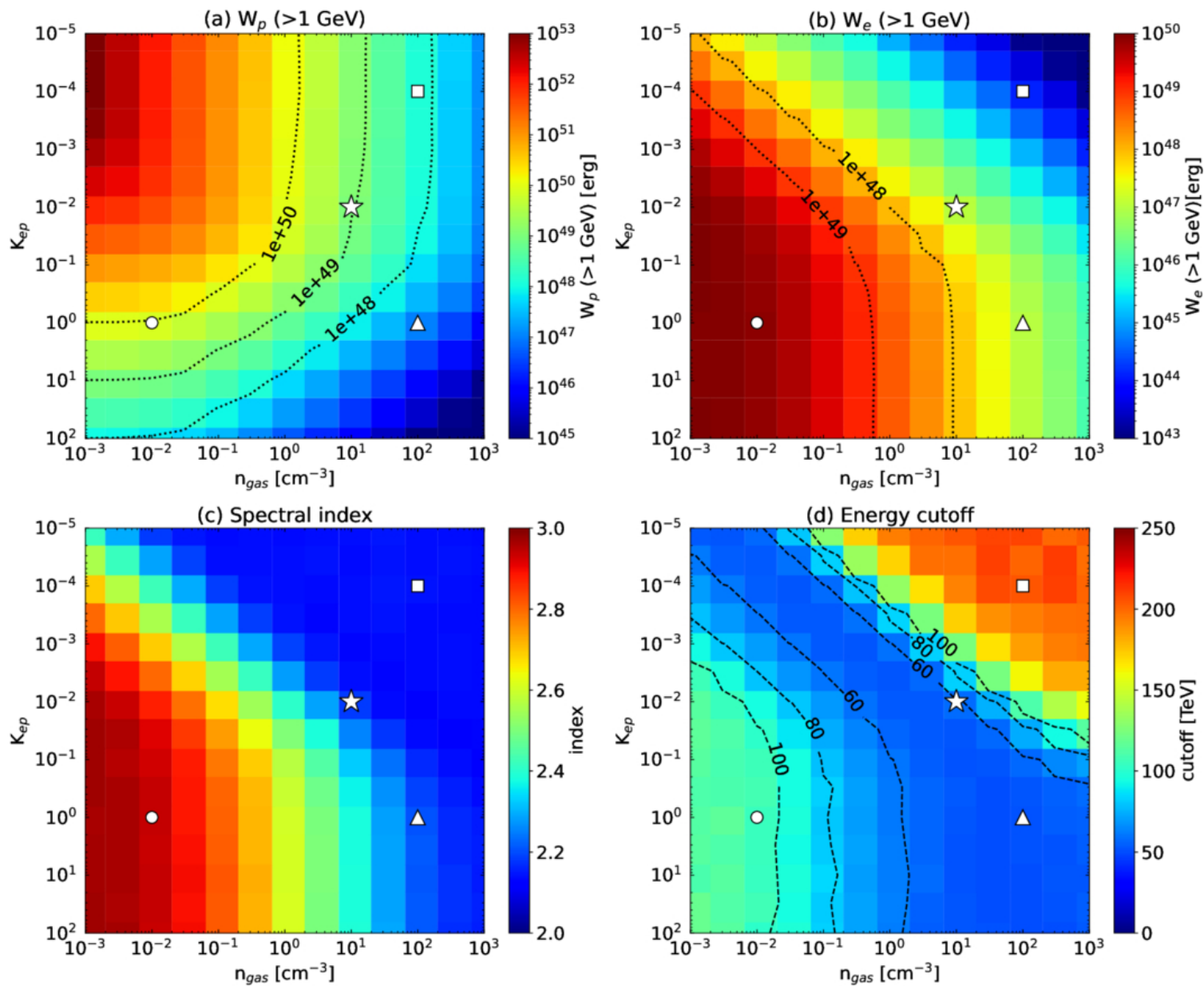
Figure 10. from Tsunefumi Mizuno et al 2026 Astrophys. J. 1006 doi:10.3847/1538-4357/ae680d https://dx.doi.org/10.3847/1538-4357/ae680d © 2026. The Author(s). Published by the American Astronomical Society.
