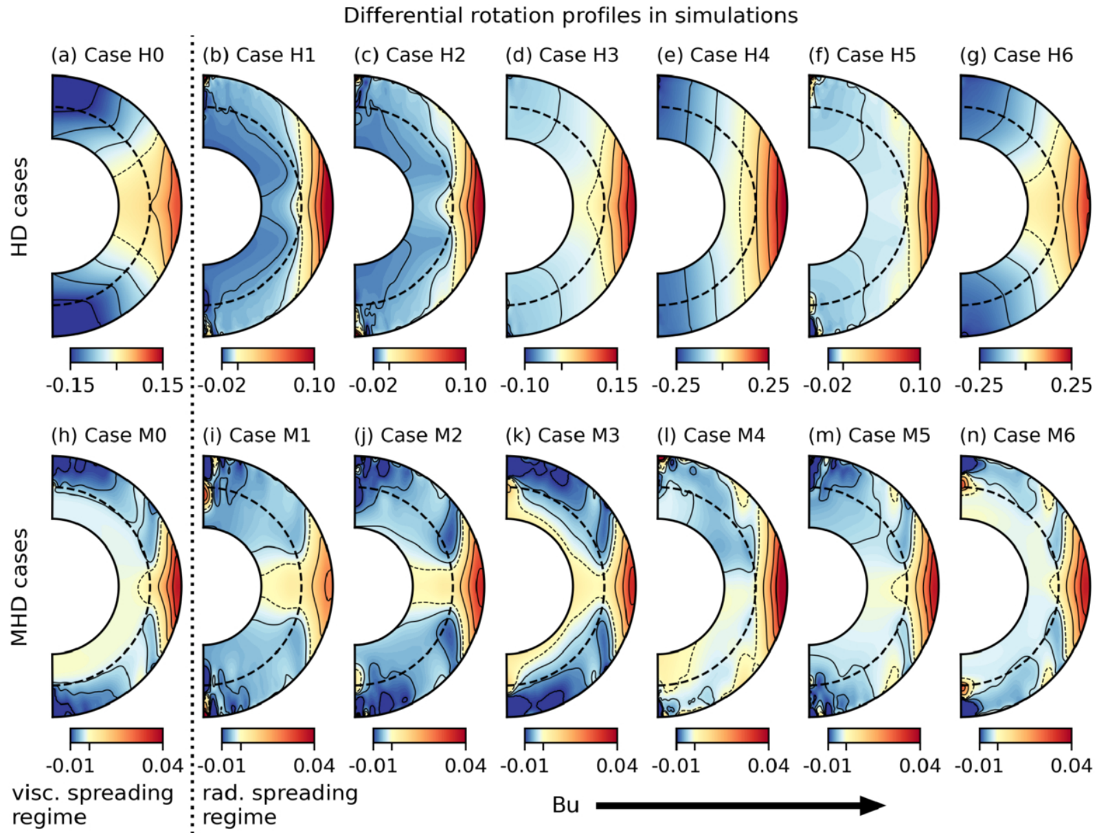
Figure 4. from Loren I. Matilsky et al 2026 Astrophys. J. 1005 doi:10.3847/1538-4357/ae6705 https://dx.doi.org/10.3847/1538-4357/ae6705 © 2026. The Author(s). Published by the American Astronomical Society.
