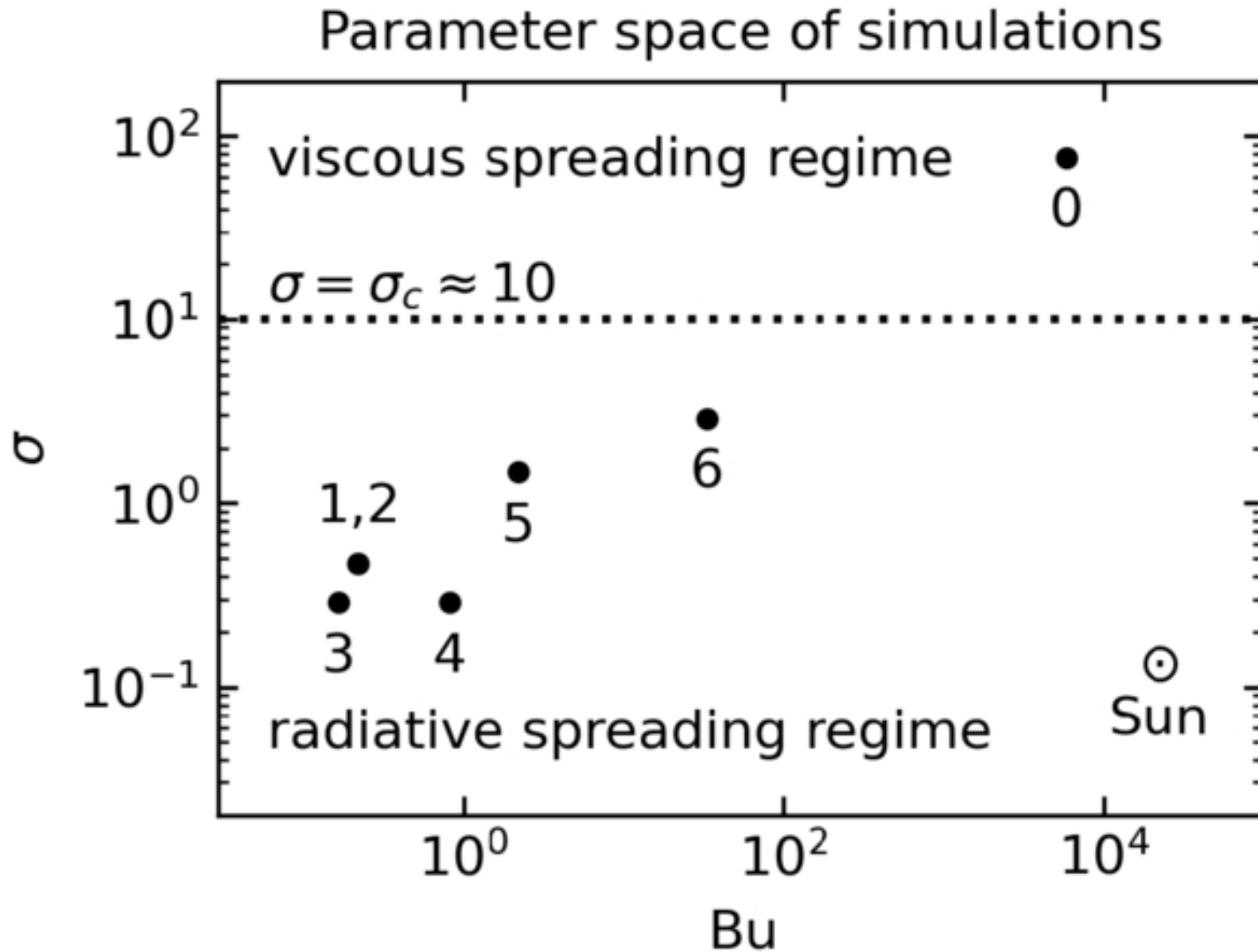
Figure 2. from Loren I. Matilsky et al 2026 Astrophys. J. 1005 doi:10.3847/1538-4357/ae6705 https://dx.doi.org/10.3847/1538-4357/ae6705 © 2026. The Author(s). Published by the American Astronomical Society.
