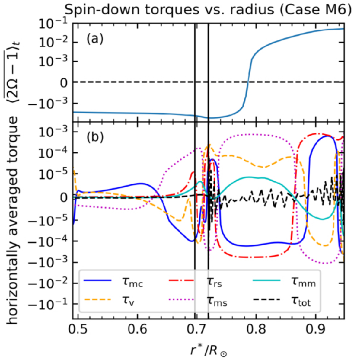
Figure 14. from Loren I. Matilsky et al 2026 Astrophys. J. 1005 doi:10.3847/1538-4357/ae6705 https://dx.doi.org/10.3847/1538-4357/ae6705 © 2026. The Author(s). Published by the American Astronomical Society.
