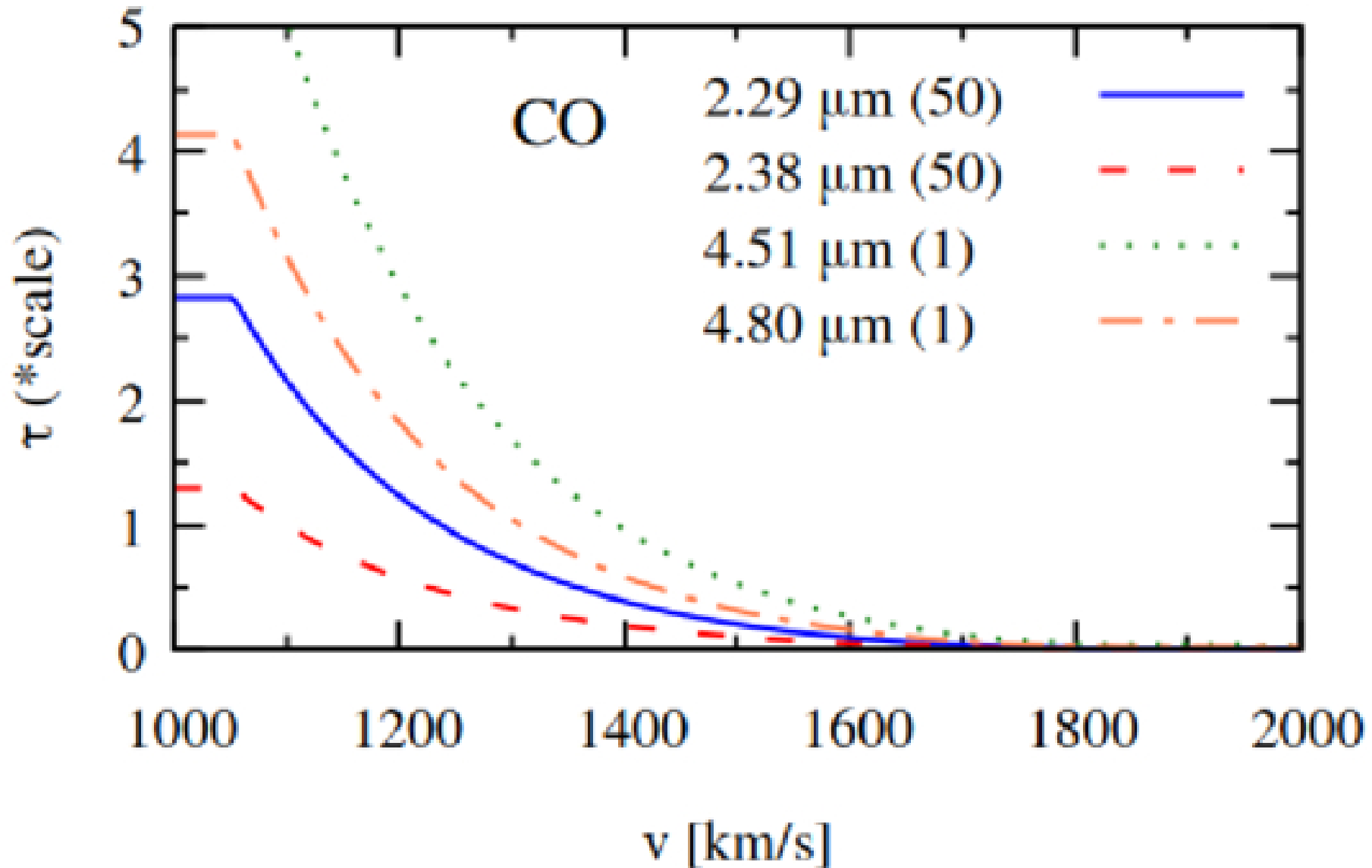
Figure 8. from T. Mera et al 2026 Astrophys. J. 1003 doi:10.3847/1538-4357/ae66ed https://dx.doi.org/10.3847/1538-4357/ae66ed © 2026. The Author(s). Published by the American Astronomical Society.
