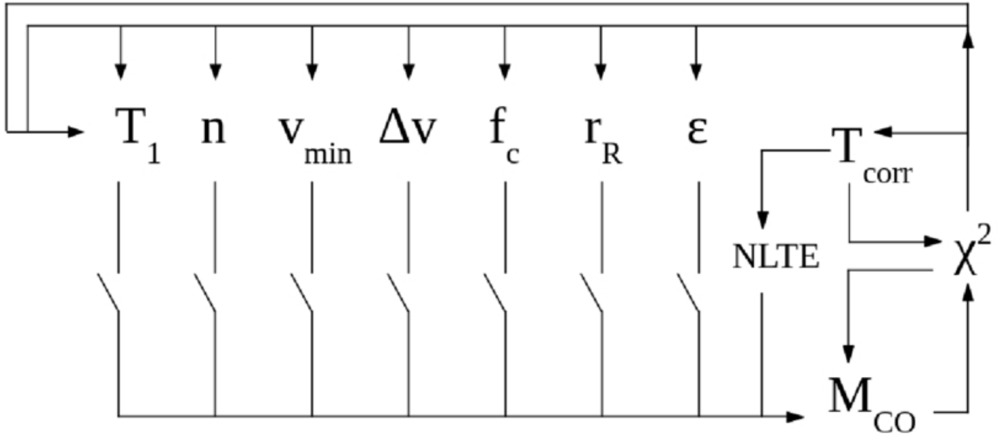
Figure 2. from T. Mera et al 2026 Astrophys. J. 1003 doi:10.3847/1538-4357/ae66ed https://dx.doi.org/10.3847/1538-4357/ae66ed © 2026. The Author(s). Published by the American Astronomical Society.
