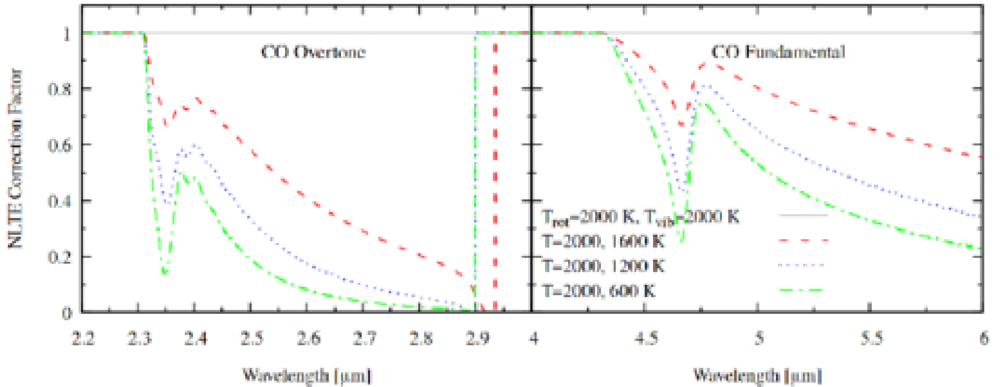
Figure 12. from T. Mera et al 2026 Astrophys. J. 1003 doi:10.3847/1538-4357/ae66ed https://dx.doi.org/10.3847/1538-4357/ae66ed © 2026. The Author(s). Published by the American Astronomical Society.
