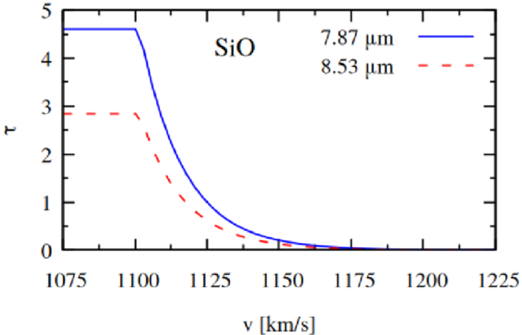
Figure 11. from T. Mera et al 2026 Astrophys. J. 1003 doi:10.3847/1538-4357/ae66ed https://dx.doi.org/10.3847/1538-4357/ae66ed © 2026. The Author(s). Published by the American Astronomical Society.
