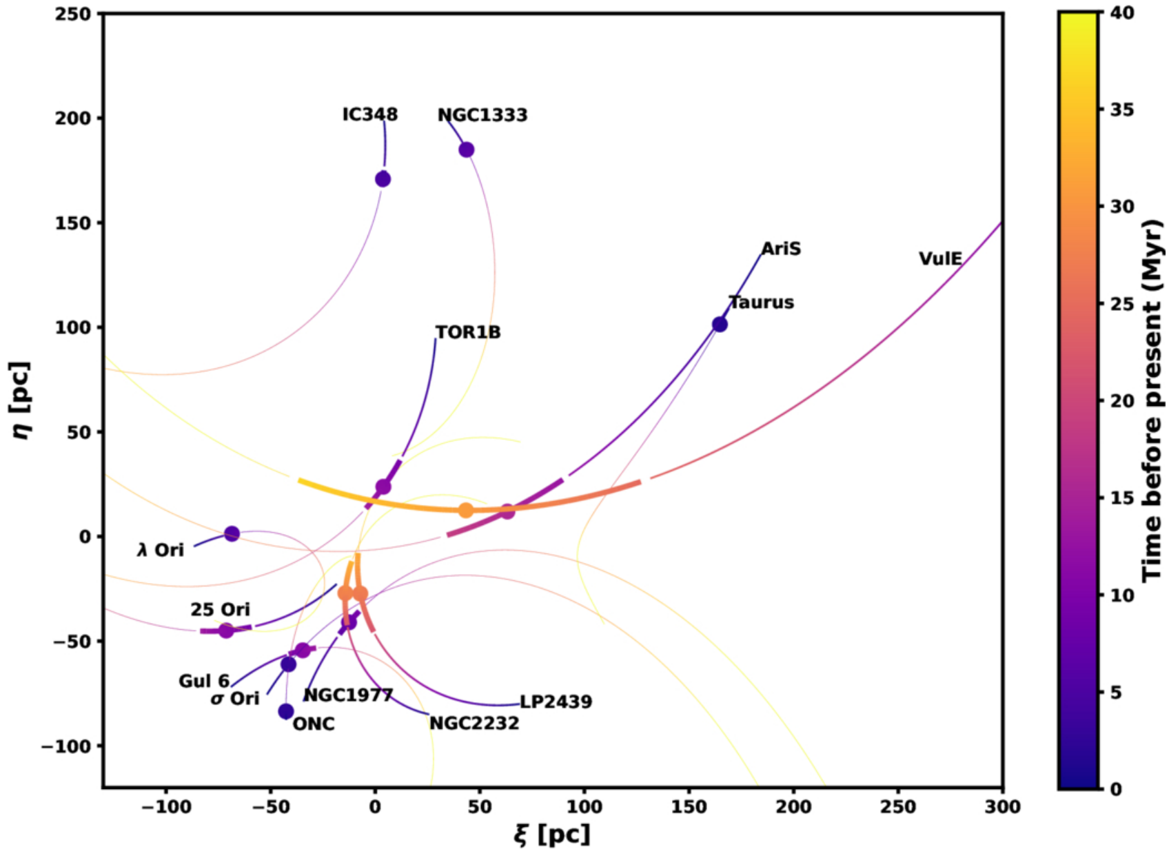
Figure 6. from Ronan Kerr et al 2026 Astrophys. J. 1004 doi:10.3847/1538-4357/ae665e https://dx.doi.org/10.3847/1538-4357/ae665e © 2026. The Author(s). Published by the American Astronomical Society.
