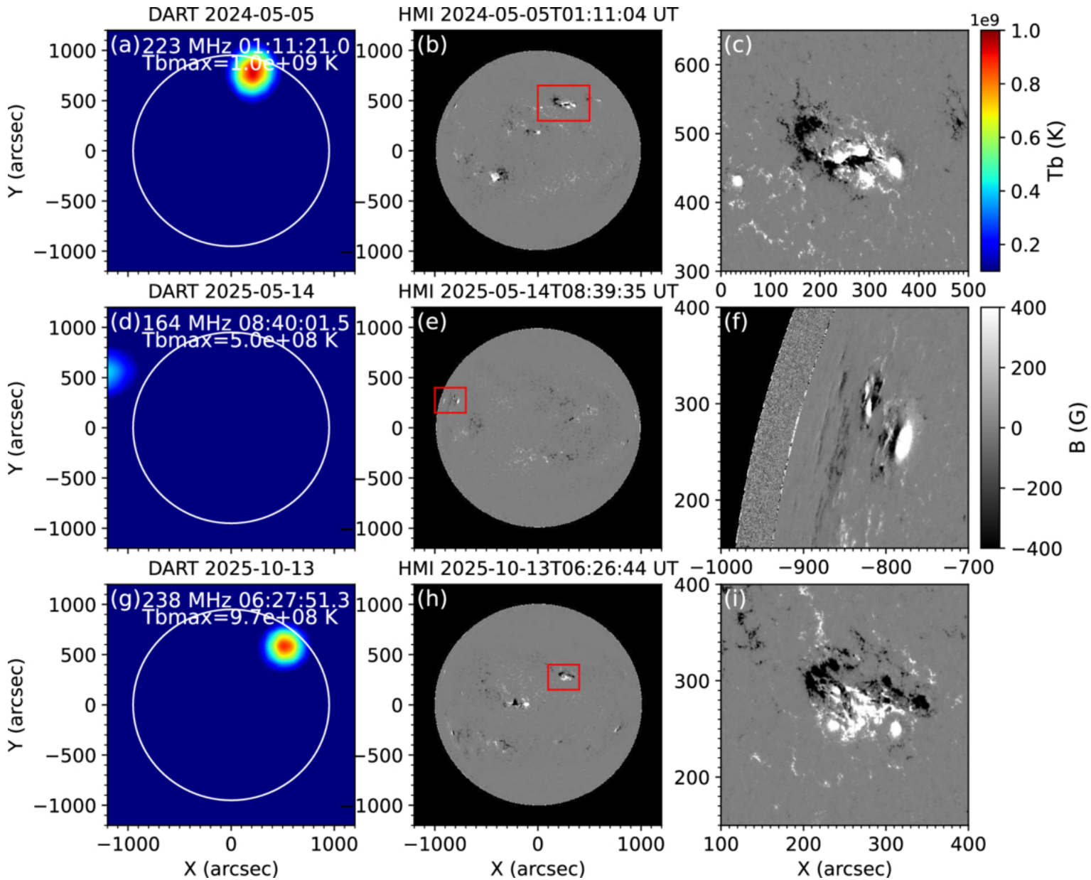
Figure 6. from Chuanyang Li et al 2026 Astrophys. J. 1003 doi:10.3847/1538-4357/ae664e https://dx.doi.org/10.3847/1538-4357/ae664e © 2026. The Author(s). Published by the American Astronomical Society.
