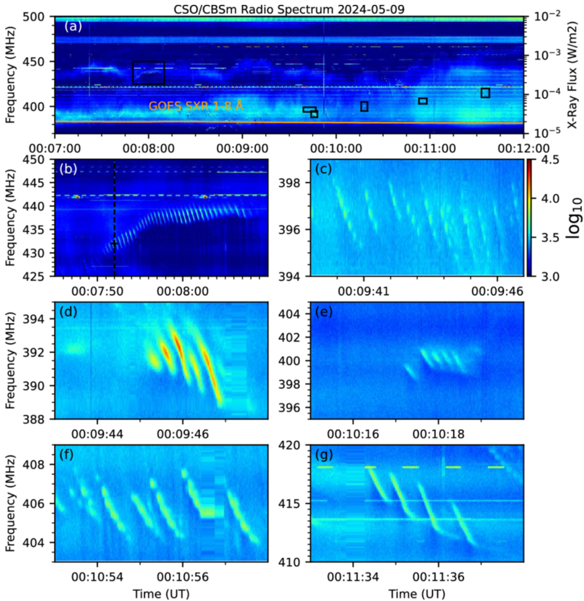
Figure 3. from Chuanyang Li et al 2026 Astrophys. J. 1003 doi:10.3847/1538-4357/ae664e https://dx.doi.org/10.3847/1538-4357/ae664e © 2026. The Author(s). Published by the American Astronomical Society.
